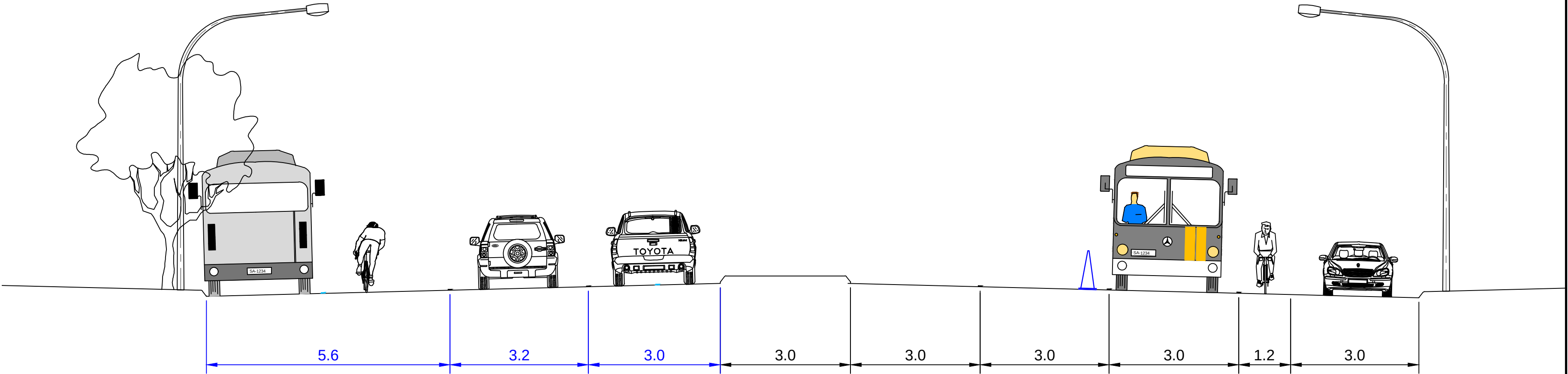
Section 1 1:75
